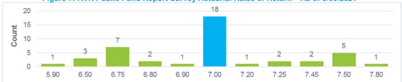
Figure 7: RVK Public Fund Report Survey Actuarial Rates of Return – As of 6/30/2021
